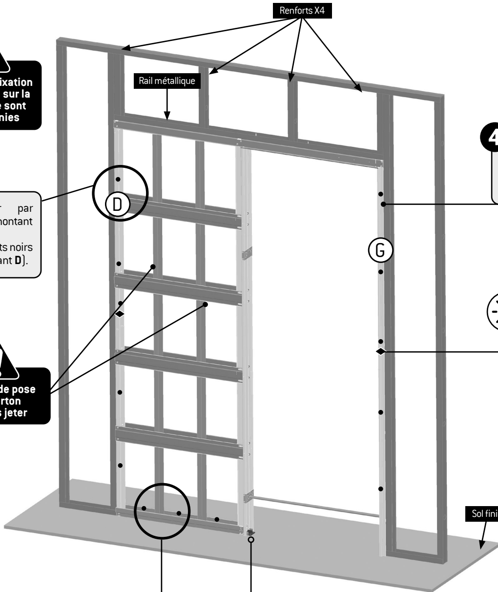
Montant M48
