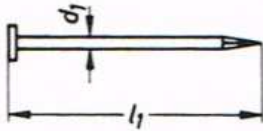
Type A, plain head
